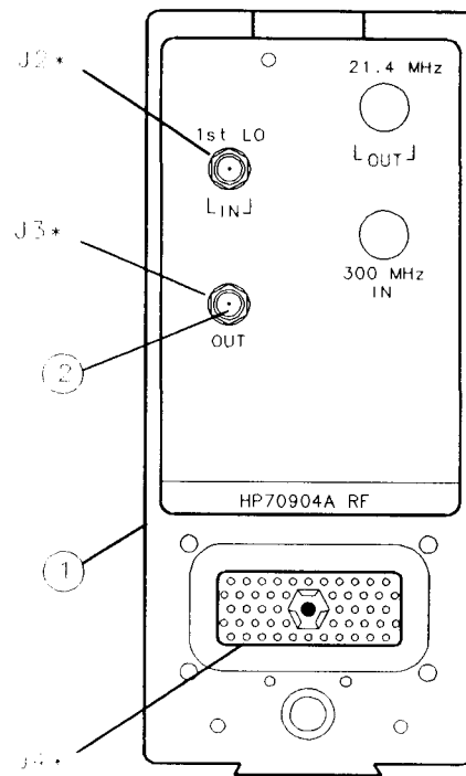
Figure 7-5. Overall Module Parts Identification, Rear Panel (1 of 2)
