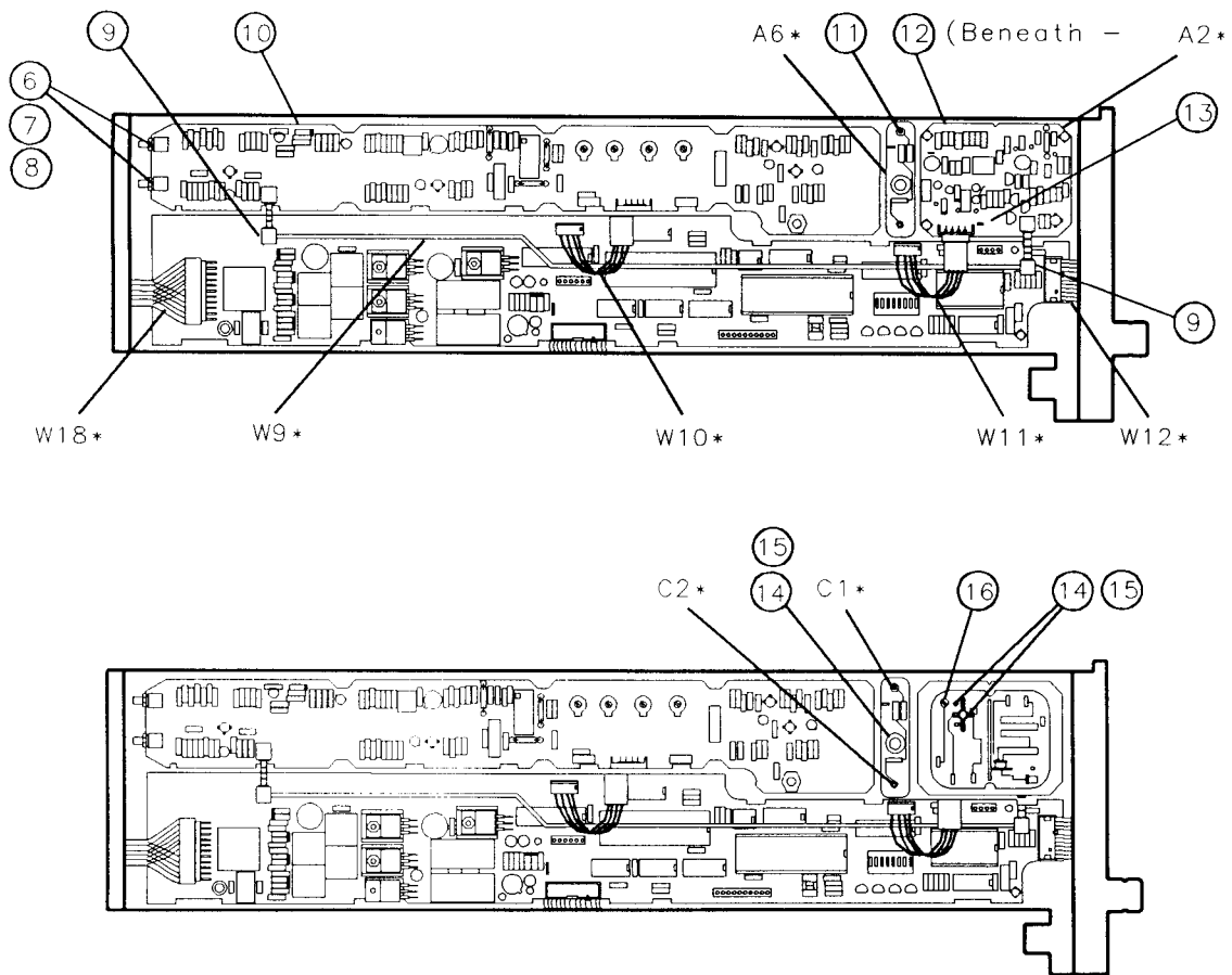
Figure 7-4. Overall Module Parts Identification, Left-Side View (1 of 2)
