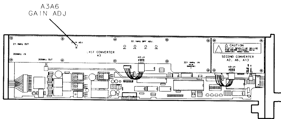
Figure 3-2. RF Flatness Gain Adjustment Location
