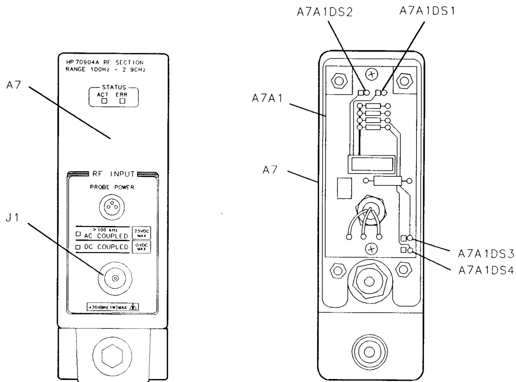
Figure 8-1. Front-Panel View, Connector and Component Designations
