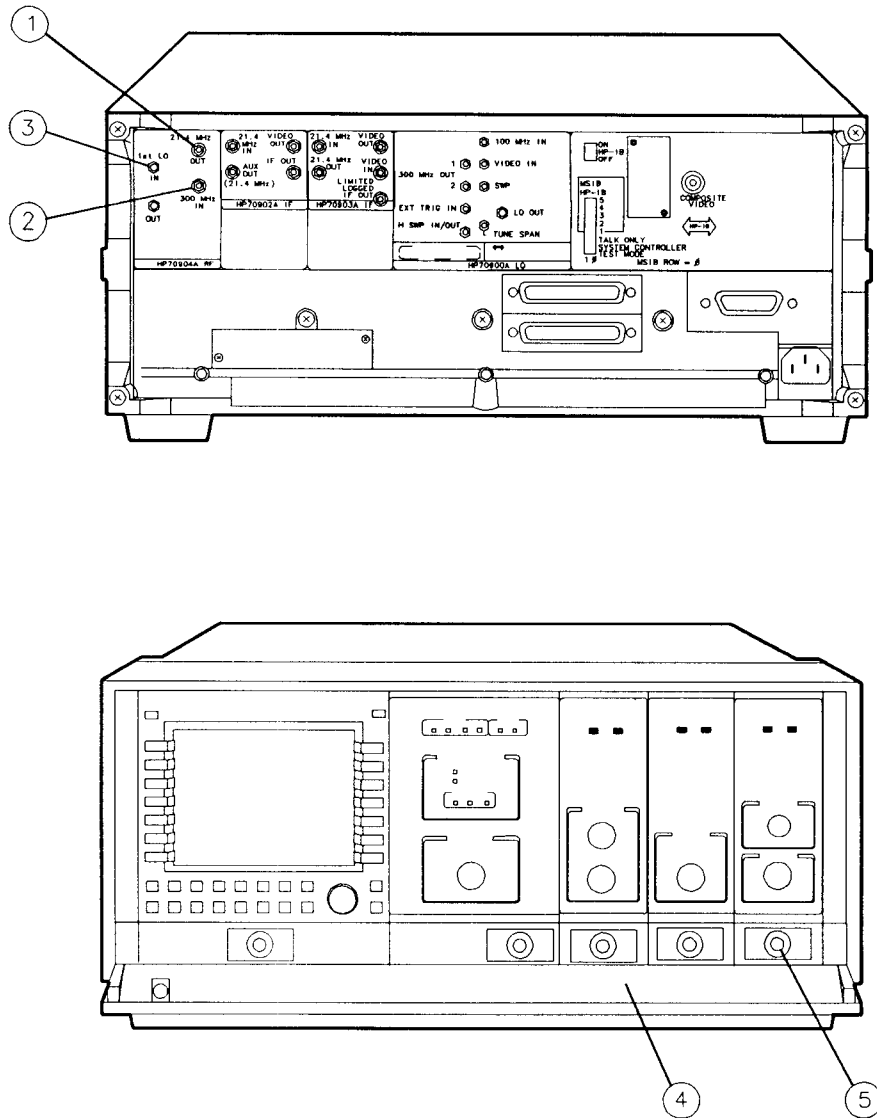
Figure 6-1. HP 70904A RF Section Replacement
