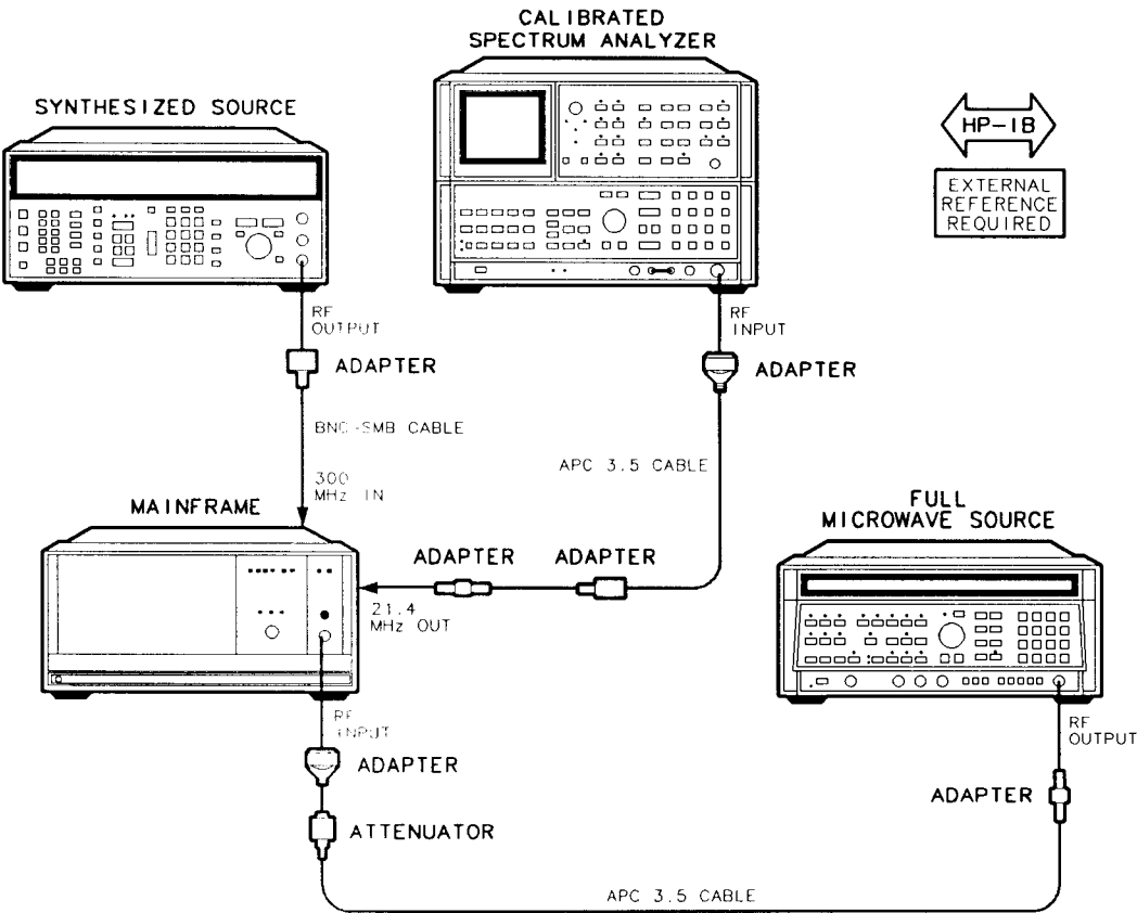
Figure 3-11. Image Rejection Test Setup
