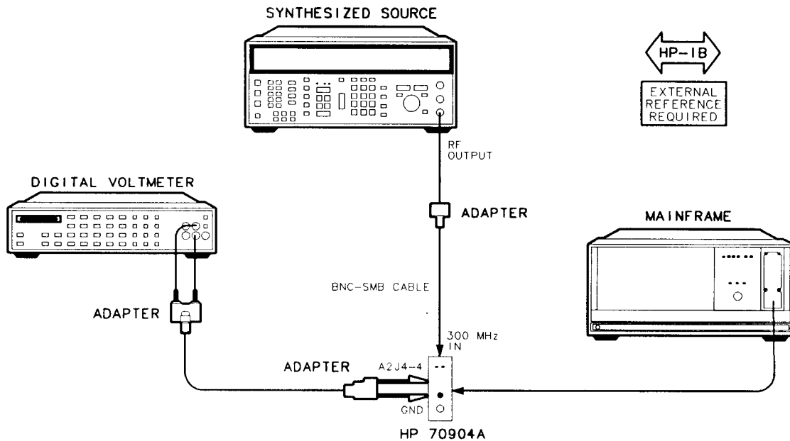
Figure 4-13. Sampler DC IF Output Check Setup
