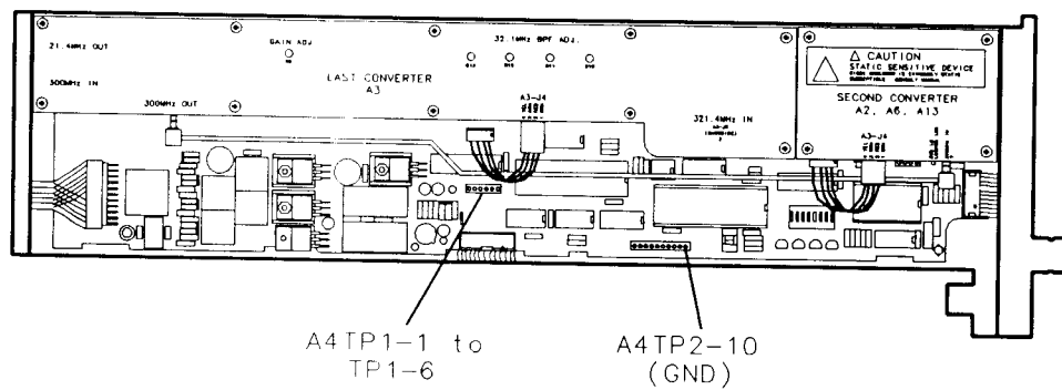
Figure 4-2. Power Supply/Controller Check
