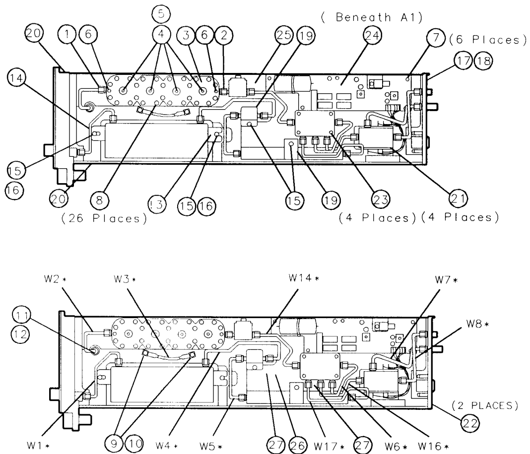
Figure 7-3. Overall Module Parts Identification, Right-Side View, Serial Prefixes 2818A and Above (1 of 2)
