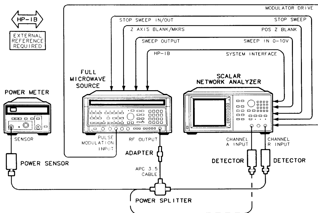
Figure 3-28. Flatness >10 MHz Calibration Setup
